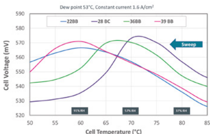
Steady-state single cell tests [RH/temperature sweep]. Cell voltages [at 1.6 A/cm 2 ] of single cells assembled with different SIGRACET GDLs
